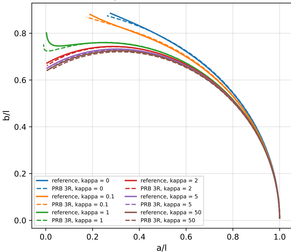
PRB 3R Model Compared with Continuous Beam Reference
